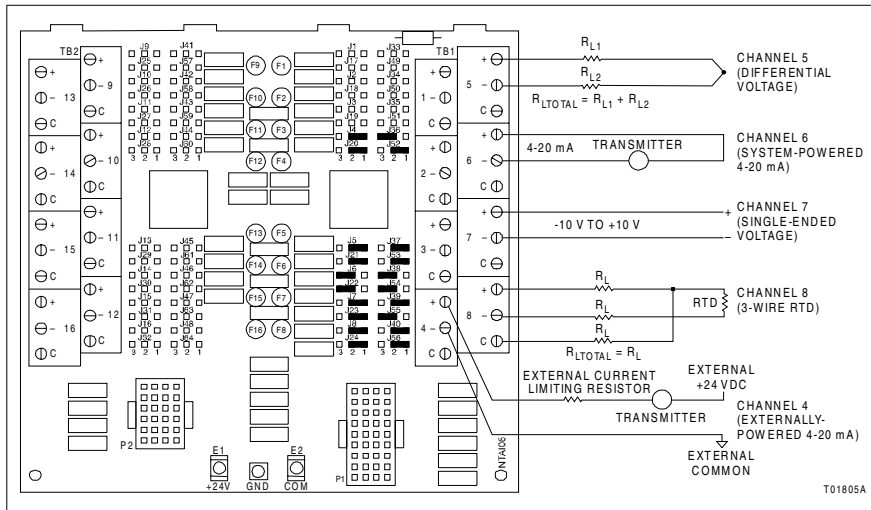
Figure A-4. NTA106 Field Input Termination Examples
